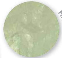
HALITE
